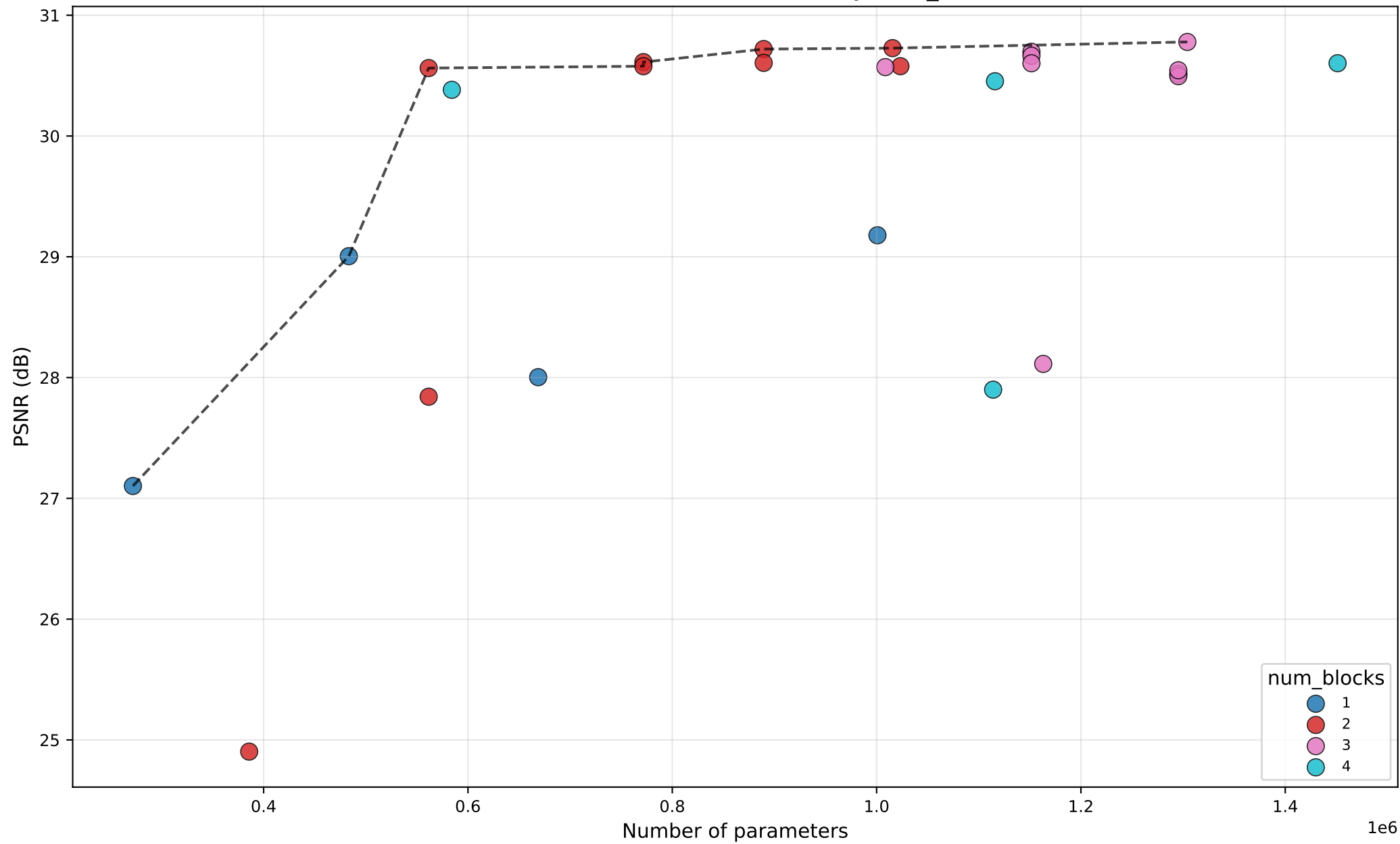
PSNR vs #Params — OmniSR — by num_blocks
